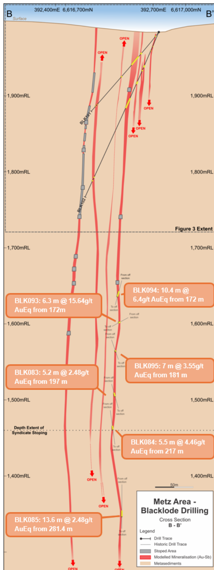
Figure 4 Blacklode Cross-section B-B'
