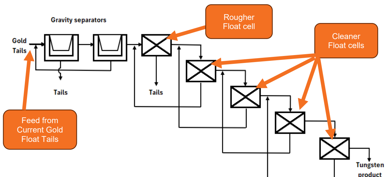
Figure 1 Proposed tungsten flotation circuit
